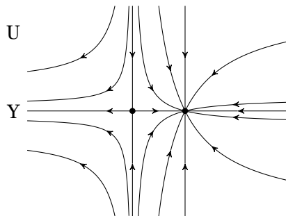
Figure 1. Example of a T -action on U \cong \mathbf{P}^1 \times \mathbf{A}^1 , t([x_0, x_1], y) = ([x_0, tx_1], ty) , with Y = \mathbf{P}^1 \times 0 shown as the horizontal line ( T = \mathbf{G}_m ). The arrows point in the direction t \rightarrow 0 . The fixed point set Y^T consists of two points.
